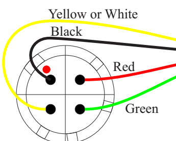
Rear View of Male Connector
